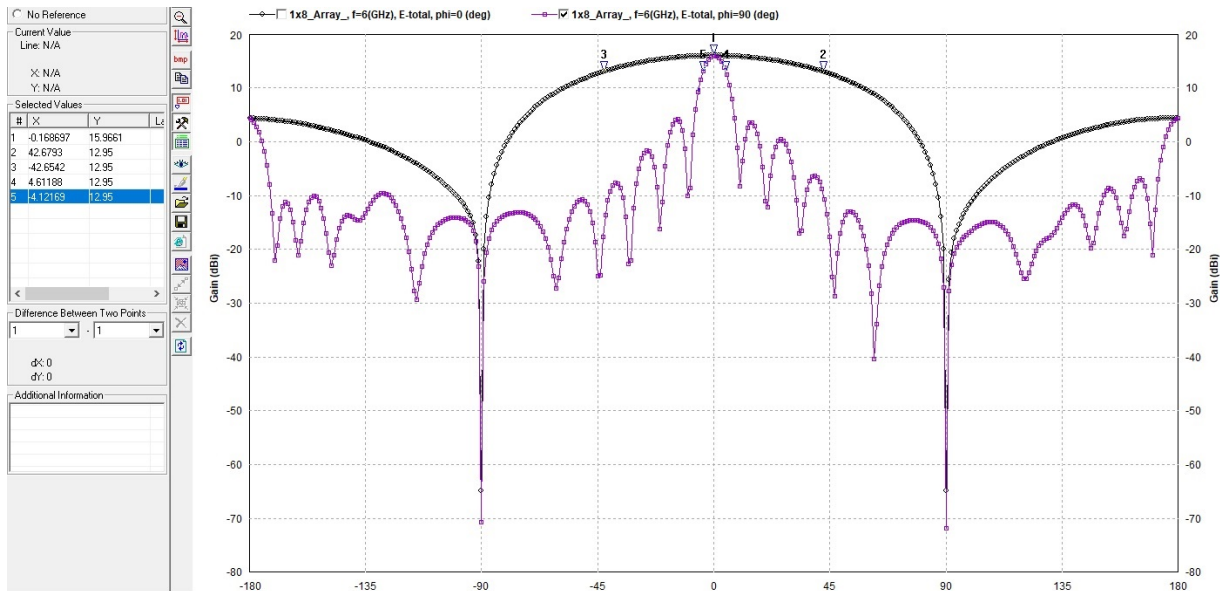
Simulate Radiation Pattern @ 6 GHz
