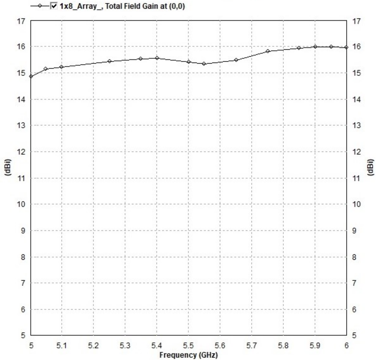
Simulated Gain plot
