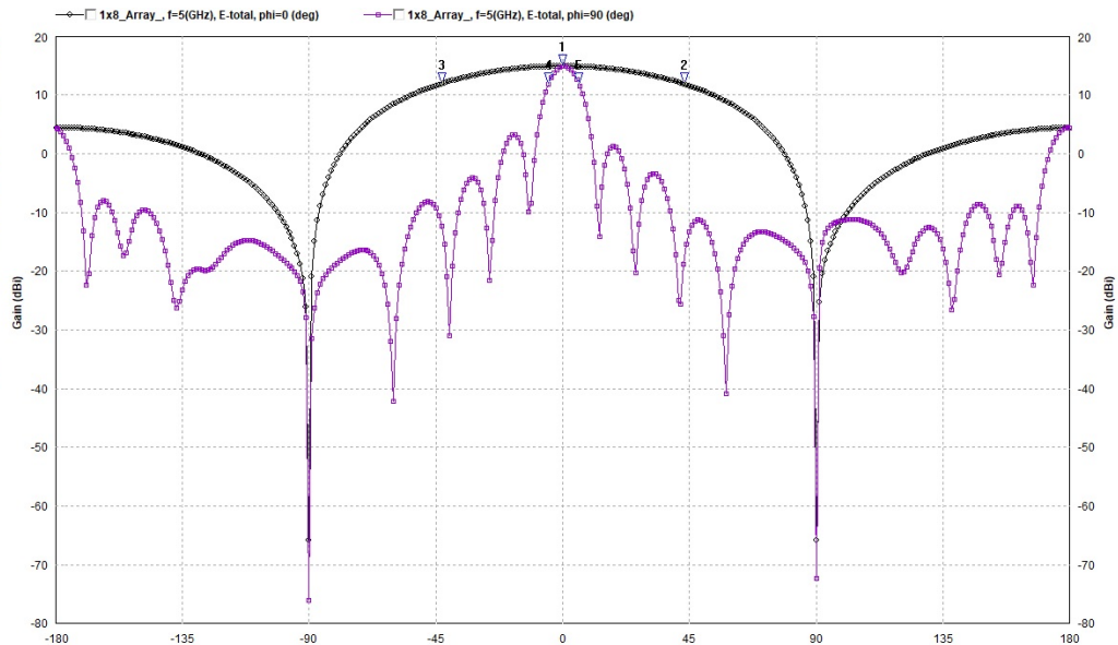
Simulate Radiation Pattern @ 5GHz
