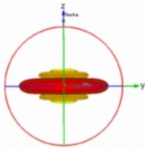
(c) Sector Antenna 3D Pattern Front View
