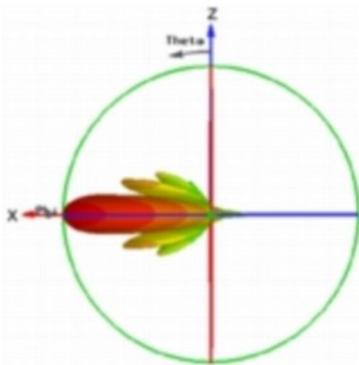
(b) Sector Antenna 3D Pattern Side View
