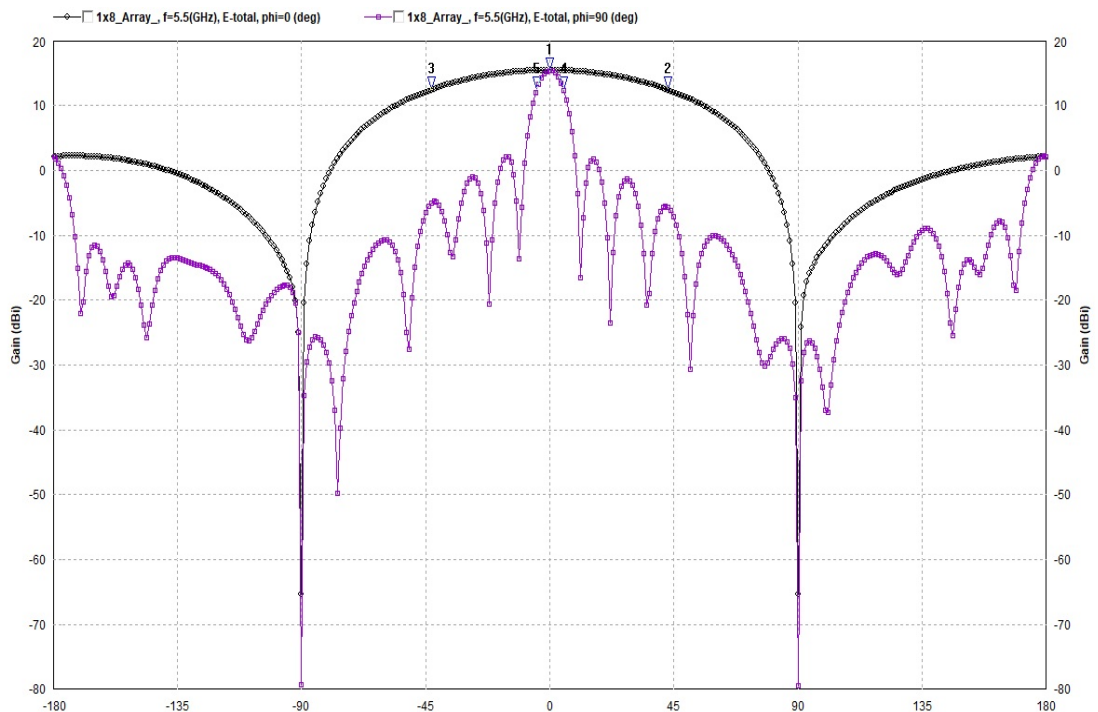
Simulate Radiation Pattern @ 5.5GHz
