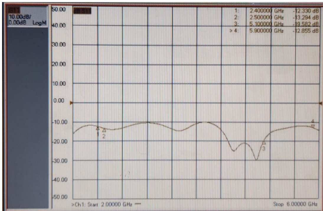
Fig 2. Return loss plot
