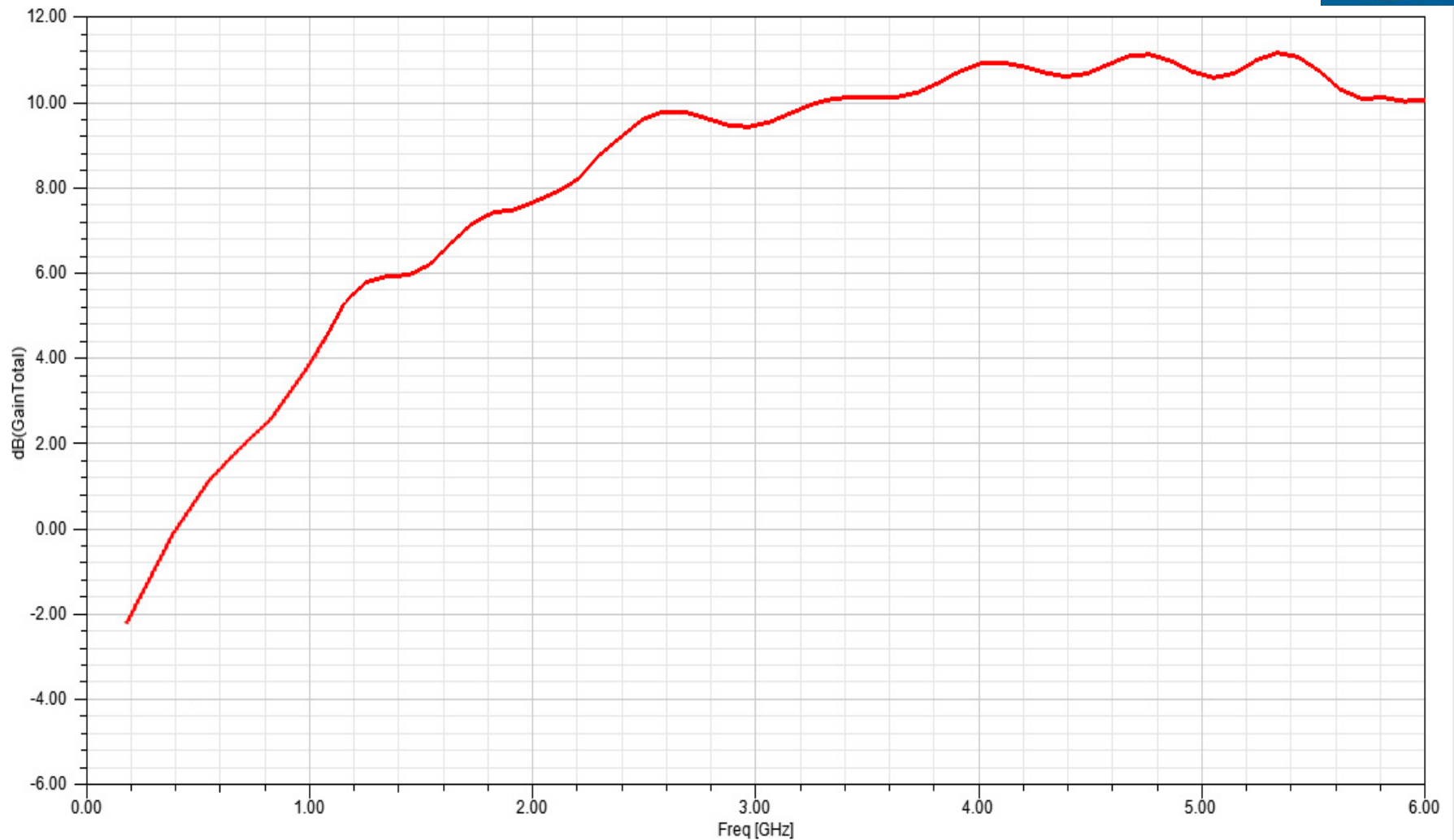
Fig3. Simulated Gain plot of the antenna
